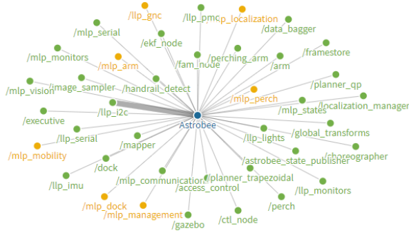
Fig. 2. Network graph of all the available Astrobbee ROS nodes.
